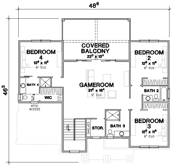
2ND FLOOR PRIMARY RESIDENCE
