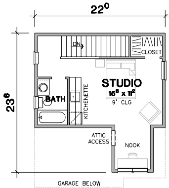
OPTIONAL GUEST HOUSE ABOVE GARAGE ADD 463 SQUARE FEET
